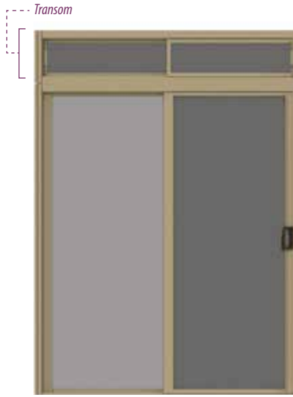
Sliding patio door with transom Widths from 60" to 106" | Door Heights from 78" to 88" Overall panel heights including Transom up to 120" Transom height with fixed glass 10" to 32" Transom height with sliding glass 14" to 32"
